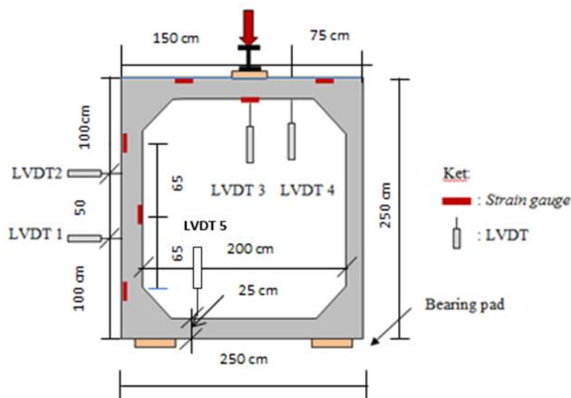
Figure 3. Location of LVDT and strain gauge.
