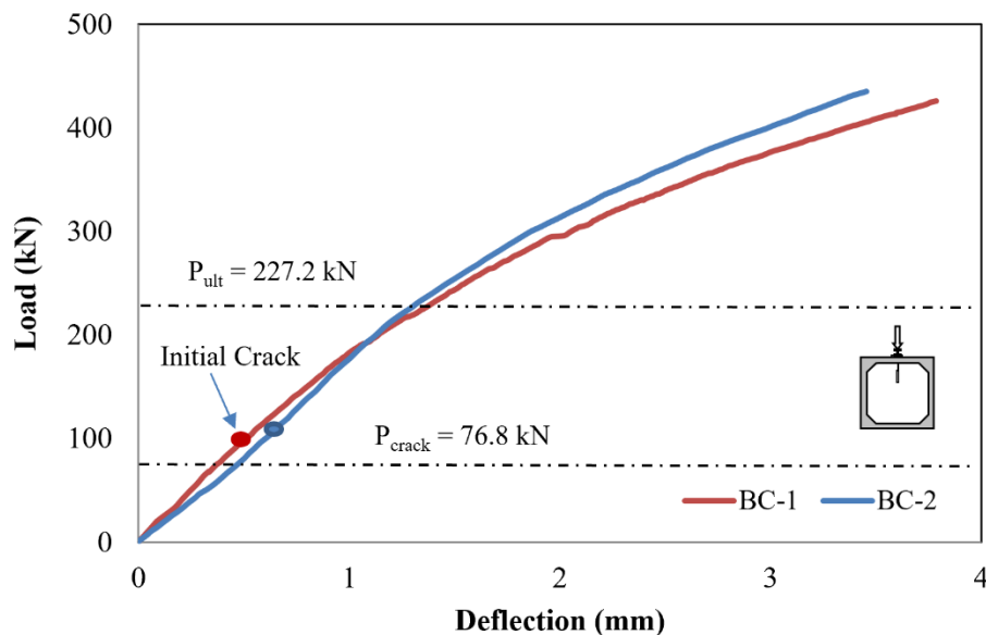
Figure 4. Load-deflection at upper wall.
