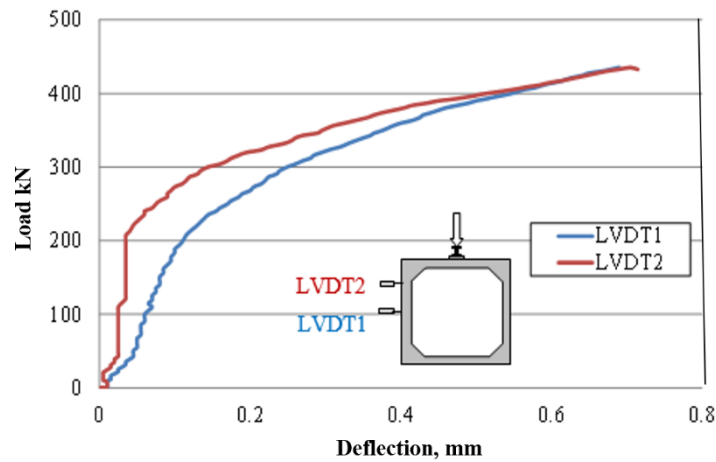
Figure 6. Load-deflection at side wall.
