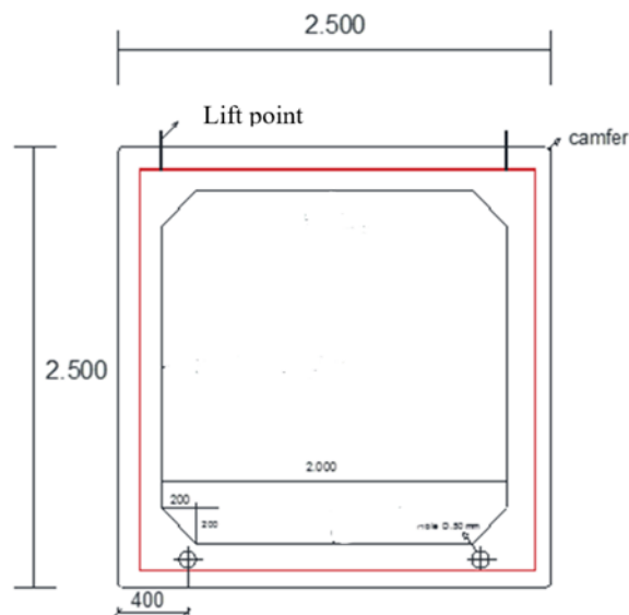
Figure 1. Dimension of box culvert.
