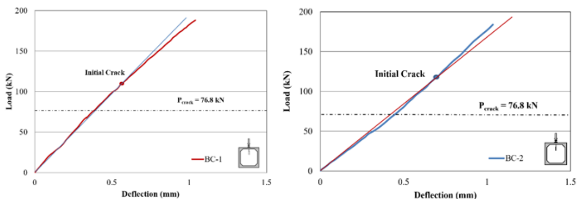
Figure 5. Initial crack of BC-1 and BC-2.
